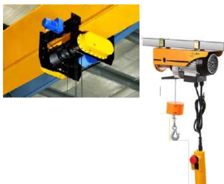
Electric Wire Rope Hoist MTC-143
